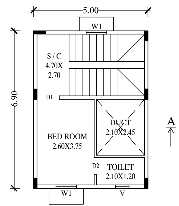
PROPOSED TYPICAL FIRST & SECOND FLOOR PLAN
