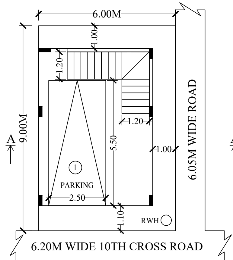
PROPOSED STILT FLOOR PLAN
